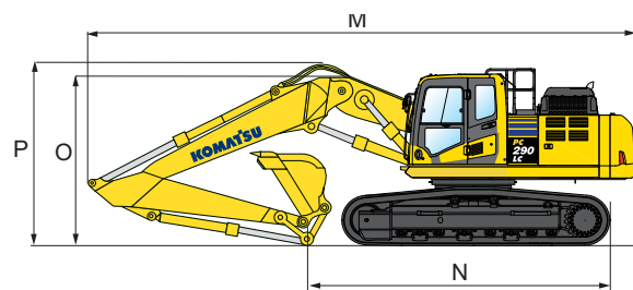
Two-piece boom
